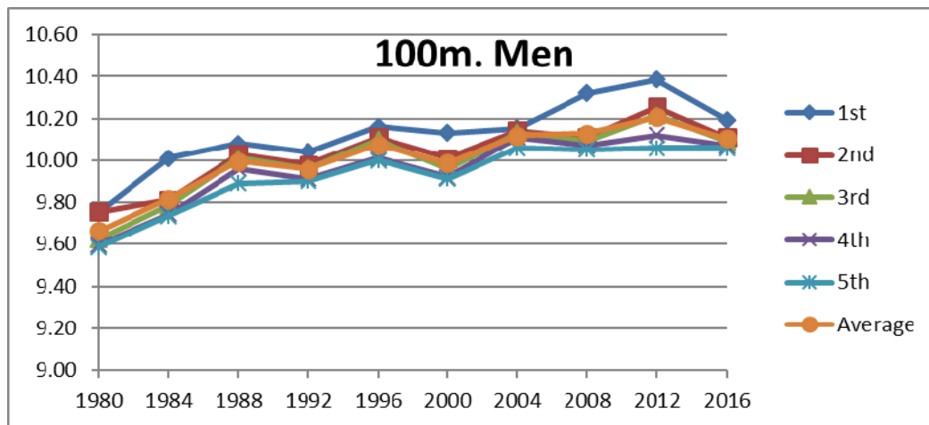
Fig 1: Graphical representation of development of 100m sprint performance for men in Summer Olympic (1980 to 2016)
