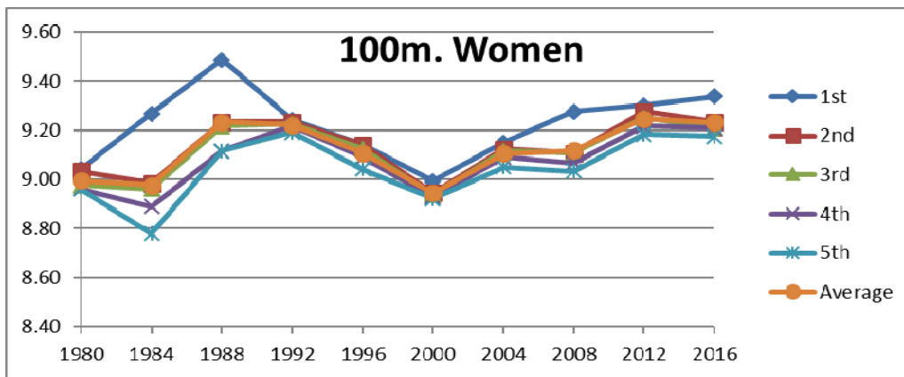
Fig 2: Graphical representation of development of 100m sprint performance for women in Summer Olympic (1980 to 2016)
