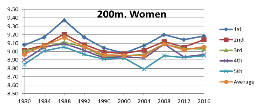
Fig 4: Graphical representation of development of 200m sprint performance for women in Summer Olympic (1980 to 2016)
