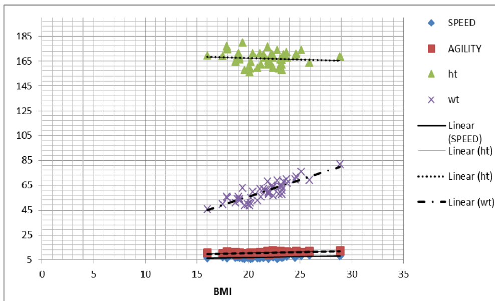
Fig 1: Graphical representation of relationship among selected variables of male Kabaddi players
